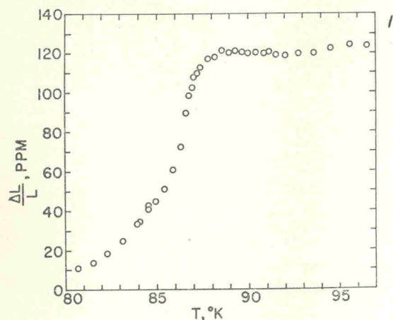
FIG. 6. Differential expansion in the vicinity of T_i for a piece of bulk, polycrystalline Eu metal about 3 \times 3 \times 20 mm long. A constant slope of 20 ppm/°K representing the sample cell expansion plus the normal Eu thermal expansion has been subtracted to emphasize the anomaly.
